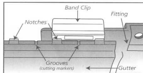
Position of lugs prior to installation, demonstrating position
