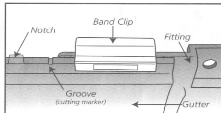
Position of gutter in Union, showing gutter fitted under clip.
