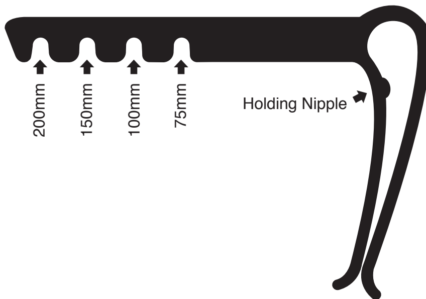
Gutterclip Profile
