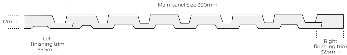
Panel and finishing trim dimensions
