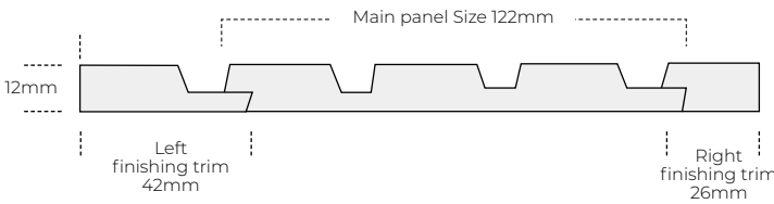
Panel and finishing trim dimensions
